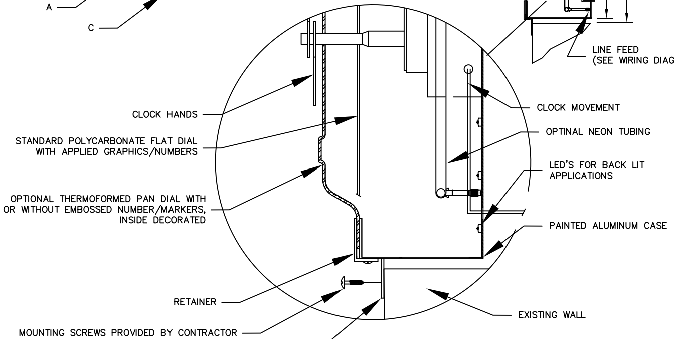
SECTION THROUGH CLOCK SHOWN WITH 2 DIAL OPTIONS
